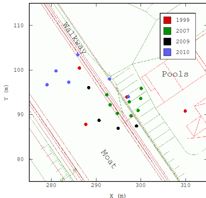
Fig. 3. Base map of the drill hole campaigns with the former map of the site.
