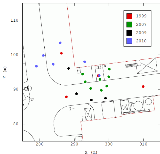
Fig. 1. Base map of the several drill hole campaigns.
