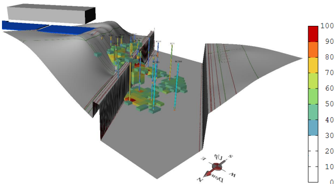
Fig. 5. Three-dimensional representation of the contamination in the former site context (topography, pools and moat). Only probabilities > 30% visible.
