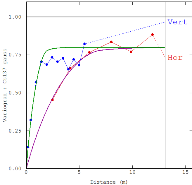
Fig. 4. Experimental variograms and corresponding models, in the horizontal plane (Hor) and in the vertical direction (Vert).
