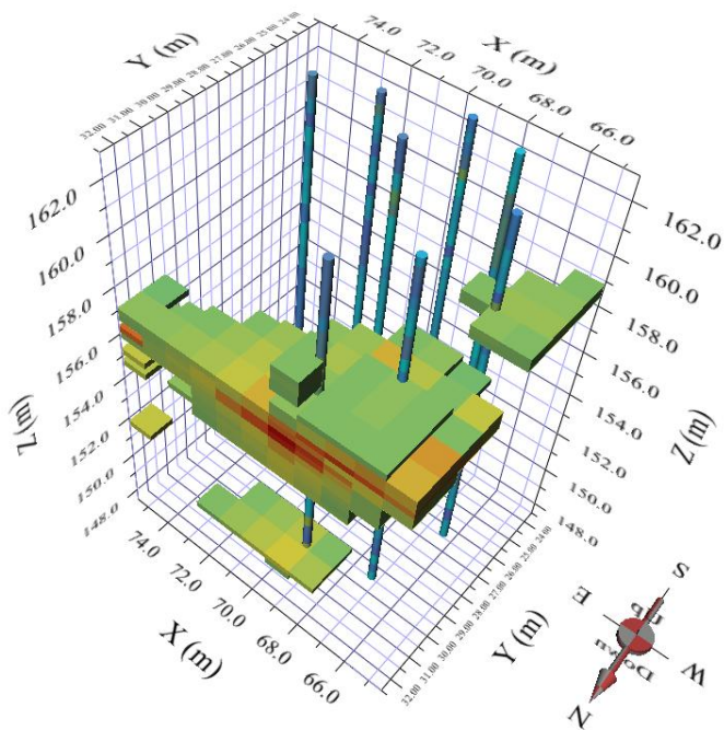
Fig. 2. Three-dimensional representation of the contamination with the first geostatistical analysis. Selection of high activity estimates (kriging).
