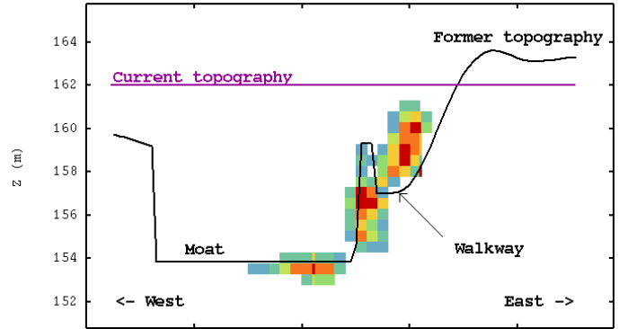
Fig. 6. Transverse section of the contamination, same color scale as Fig. 5 (vertical scale x2).
