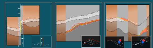
Fault uncertainty
